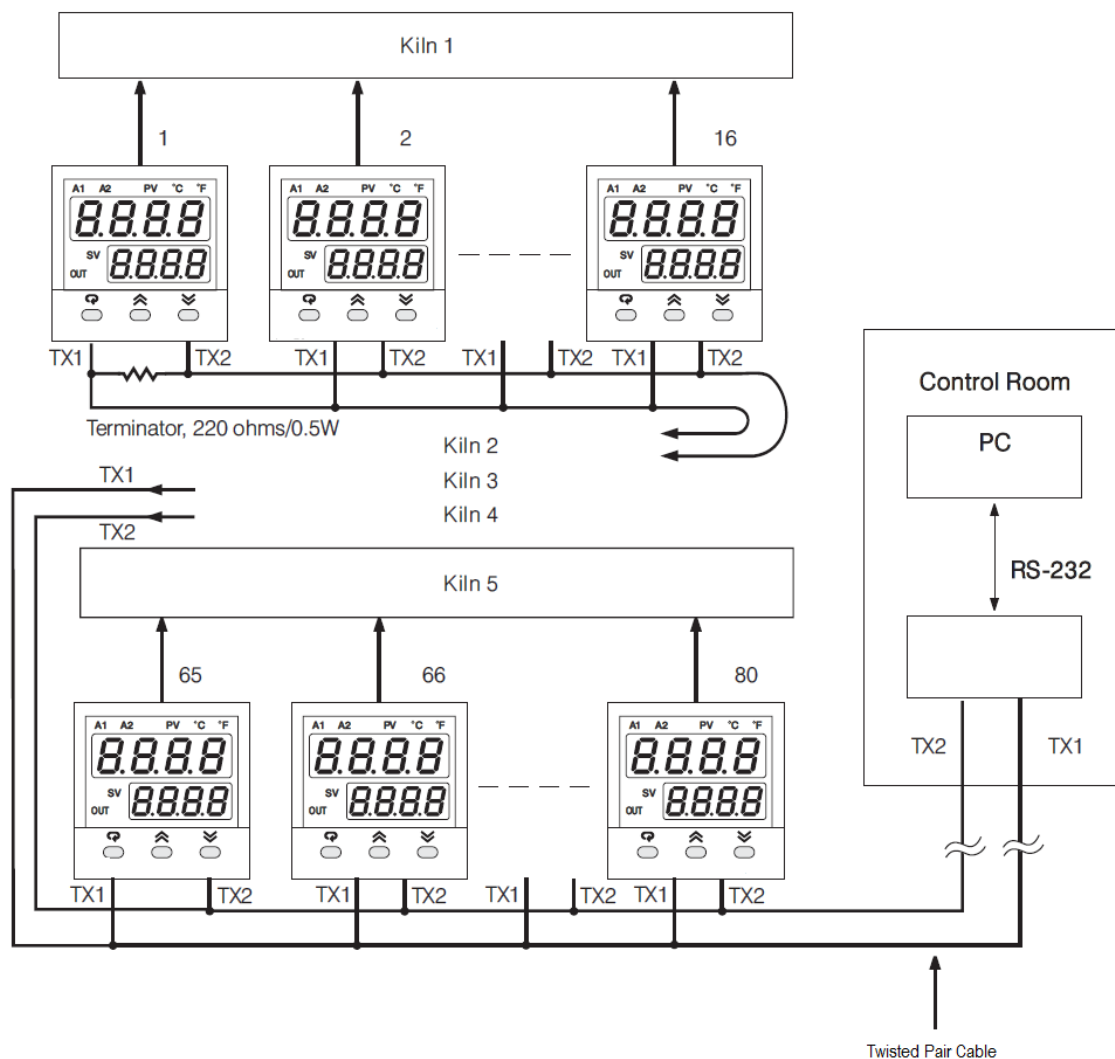
4-9.RS-485 Application
